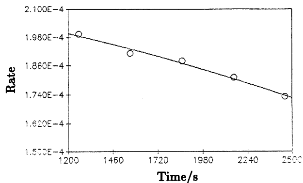
Fig. 6. Plot of first order rate ( k_\psi ) versus time for the oxidation of styrylpyridinium dye ( 3 ) by CTAP at 30^\circ\text{C} .
